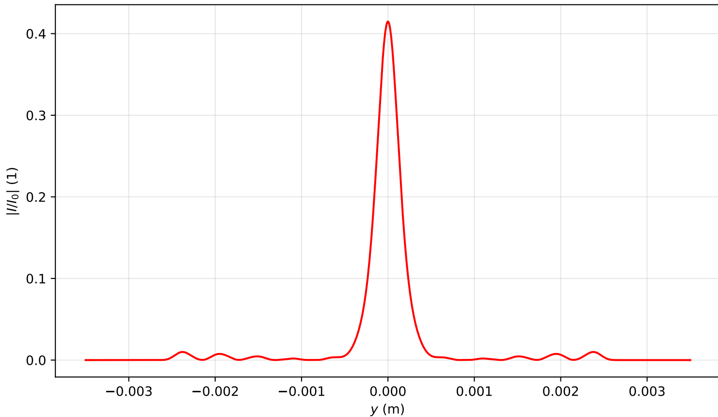
Intensity profile I(x=0, y, z=2.707)/I_0 , P_{in}=8.0P_{cr} , artificial time
